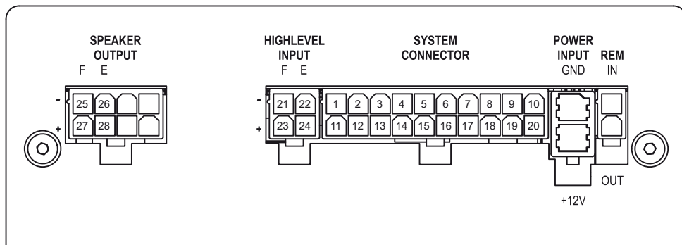
Fig. 1: Pin configuration UP 6DSP
